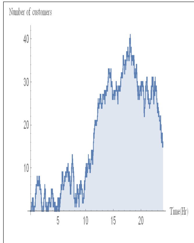
Figure 2: Simulation of M/M/2 queue model Arrival rate
