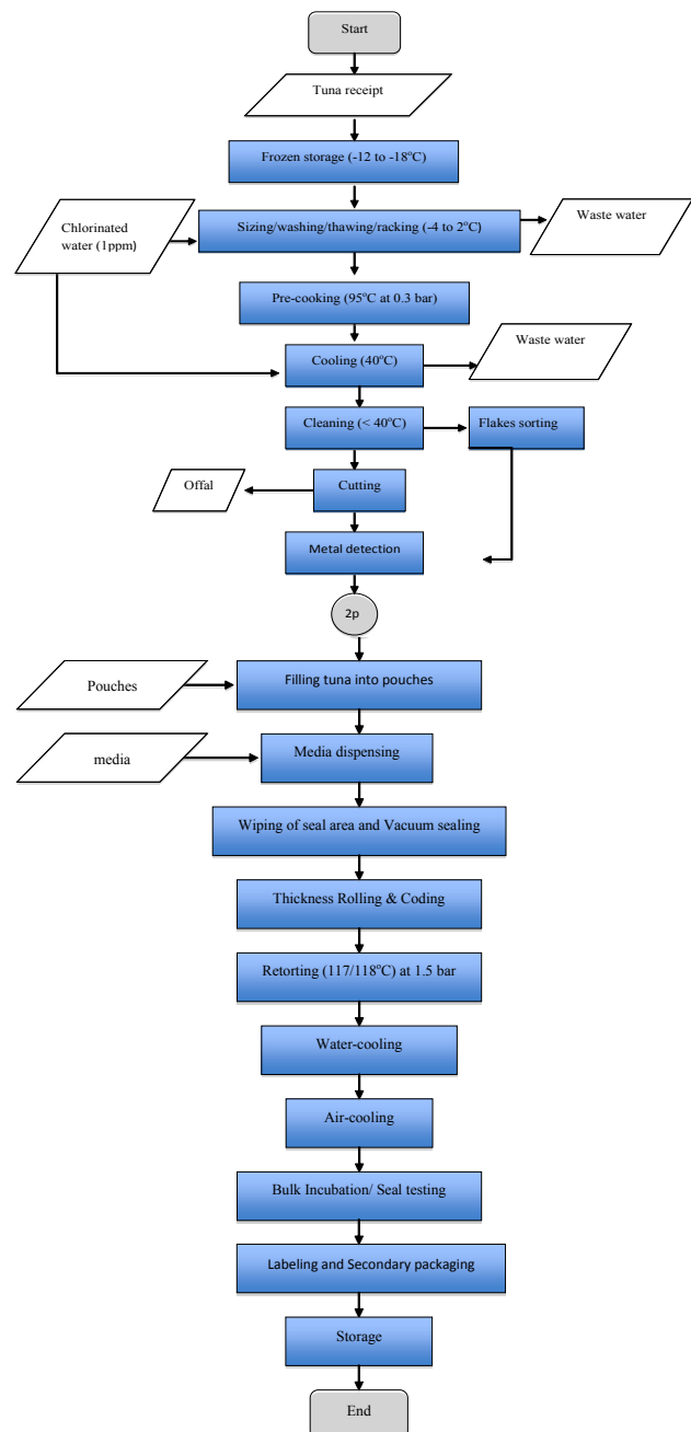
Figure 1. Flow chart for processing of vacuum-packed pouched tuna chunks
