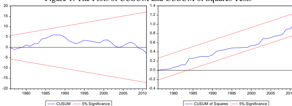
Figure 1: The Plots of CUSUM and CUSUM of Squares Tests
